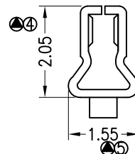
SEC:C-C
