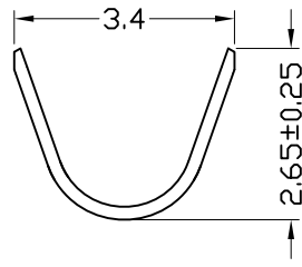
SCETION:A-A
