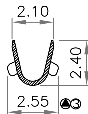
C-C Section
