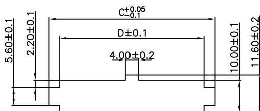
RECOMMENDED PANEL HOLE DIMENSION (THICKNESS:0.8~2.0)
