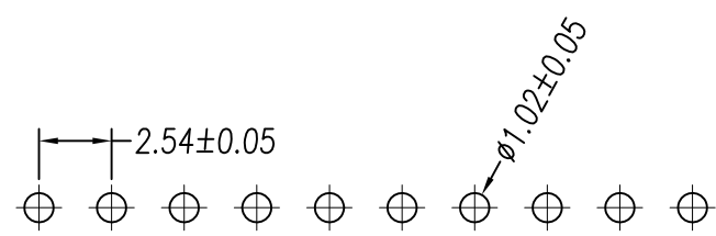
Recommended PCB Board Hole Layout
