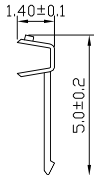
B-B SECTION
