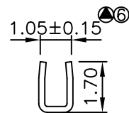
SEC:C-C
